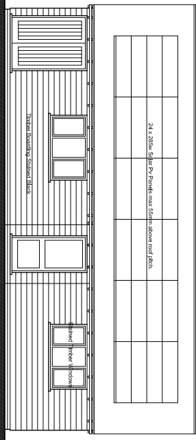
Front Elevation
